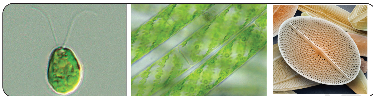
(a) Chlamydomonas
