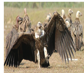
vulture
