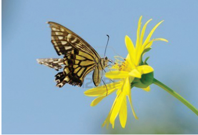
Fig-6 Butterfly
