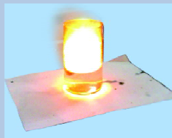
Fig. 4.5 : Reaction of sodium with water
