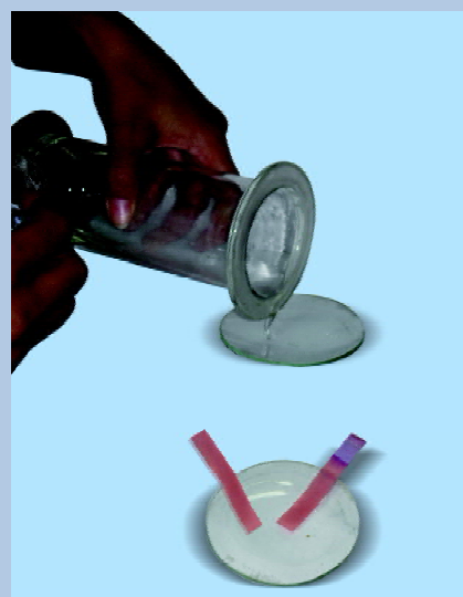
Fig. 4.4 (b) : Testing of solution with litmus papers
