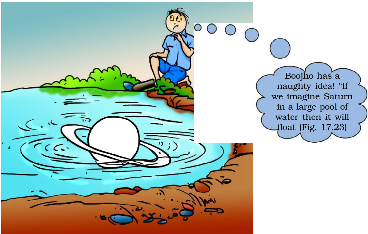
Fig. 17.23 : Saturn is less dense than water
