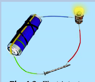
Fig. 4.2 : Electric tester
