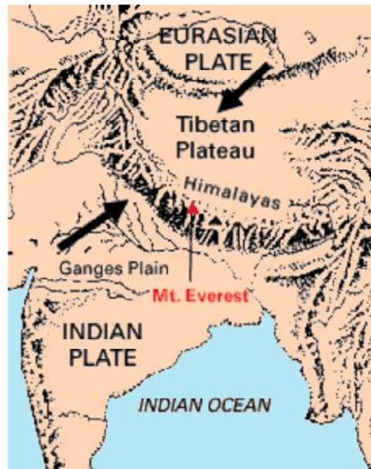
Fig. 15.12 : Movements of Indian earth's plate
