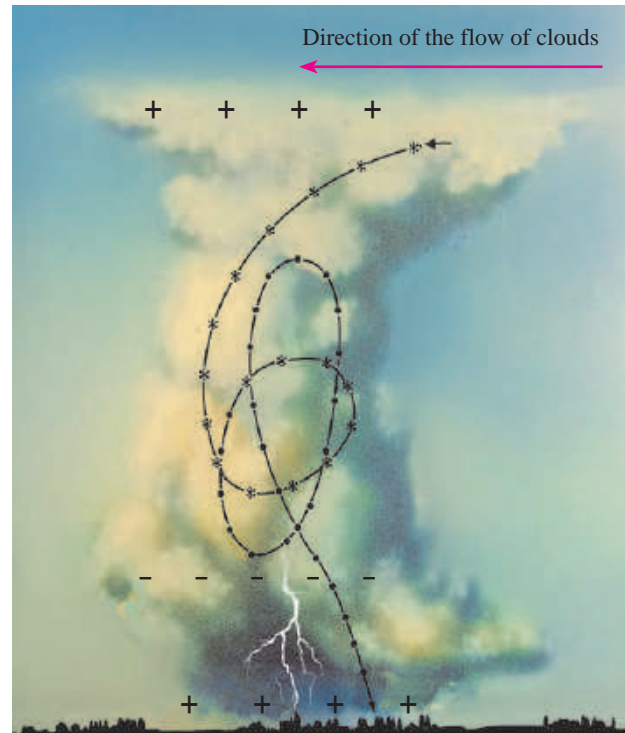
Figure 3.9 : Cumulonimbus Clouds
