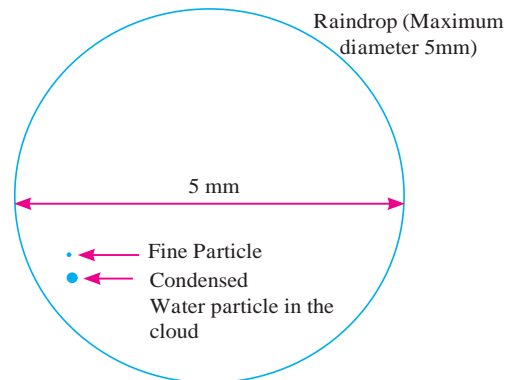
Figure 3.7 : Raindrop
