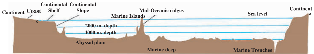
Figure 4.2 : Ocean relief
