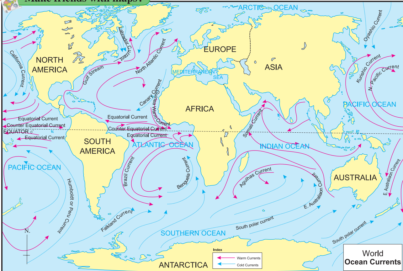
Figure 5.4 : Ocean Currents
