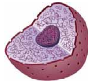
Fig. 1.7 Nucleus
