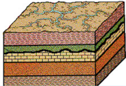
Fig. 4.35: Disconformity
