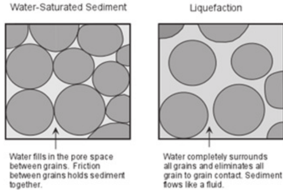
Fig. 7.16: Effects of liquefaction in water saturated sediments
