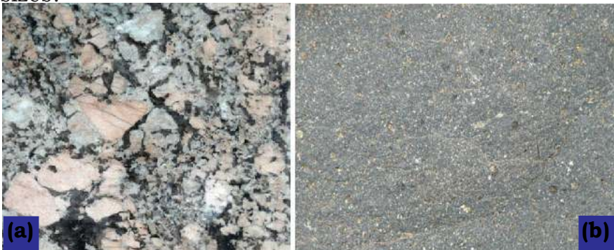
1.4 : (a) Phaneritic texture and (b) aphanitic texture
