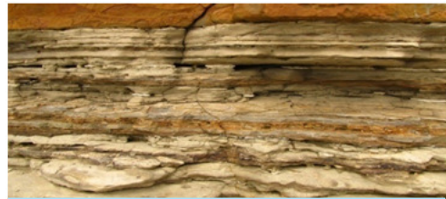
Fig. 4.10: Bedding or stratification
