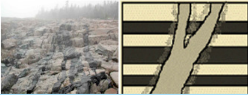
Fig.5.8 : (a) igneous intrusions in an outcrop (b) in cross section
