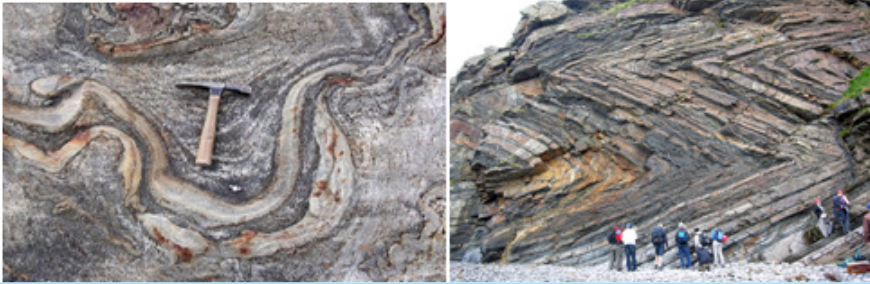
Fig. 4.11: Folds in rocks
