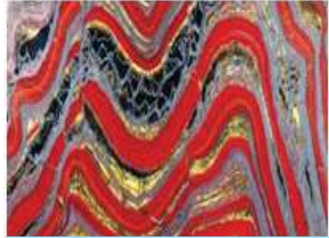
Fig.2.6: Banded iron formations
