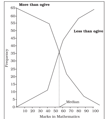
Fig. 4.8(b): 'Less than' and 'More than' ogive for data given in Table 4.10
