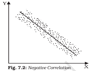
Fig. 7.2: Negative Correlation
