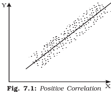
Fig. 7.1: Positive Correlation
