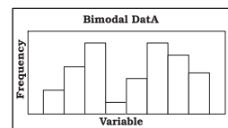
Bimodal Data
