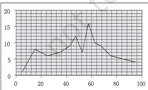
Fig. 3.2: Frequency Curve
