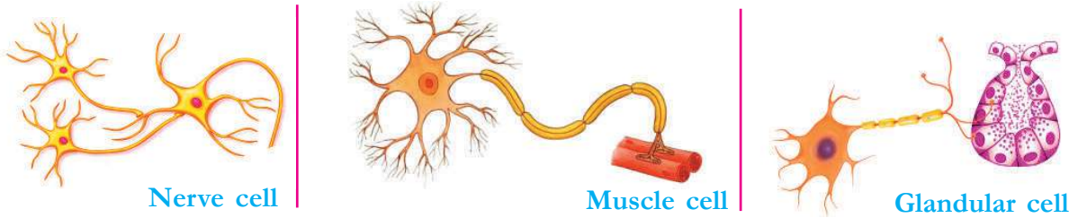
Illustration 1.5 Different types of synapses
