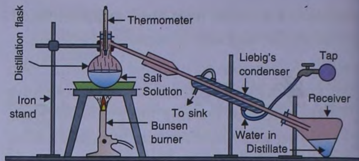
Fig. 5.5 Distillation
