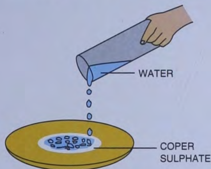
Fig. 5.11: Adding water to white copper sulphate turns them blue
